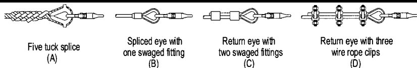
Figure 9 - Subsystem Assemblies
