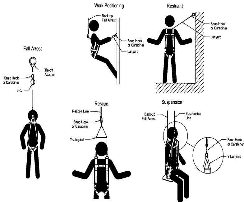
Figure 2 - Snap Hook & Carabiner Applications
