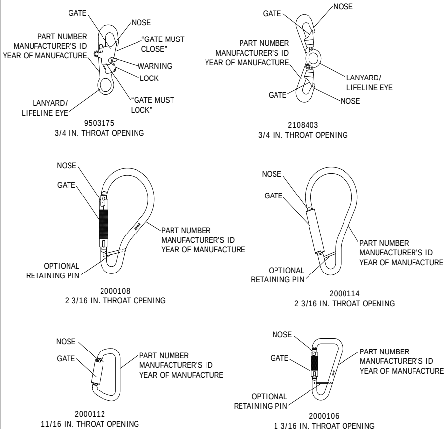
Figure 1 - Snap Hooks and Carabiners
