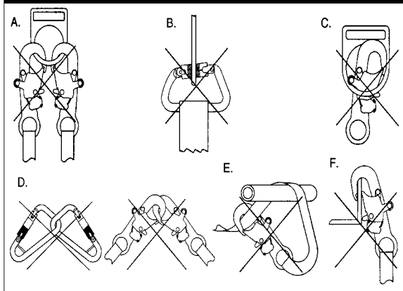
FIGURE 5 - INAPPROPRIATE CONNECTIONS
